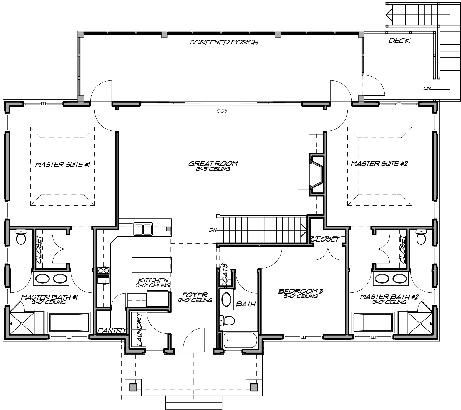
MAIN LEVEL PLAN
