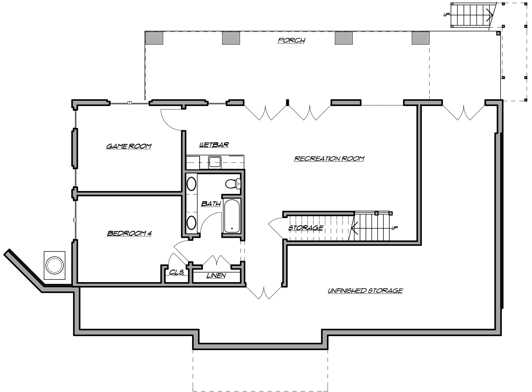
TERRACE LEVEL PLAN
